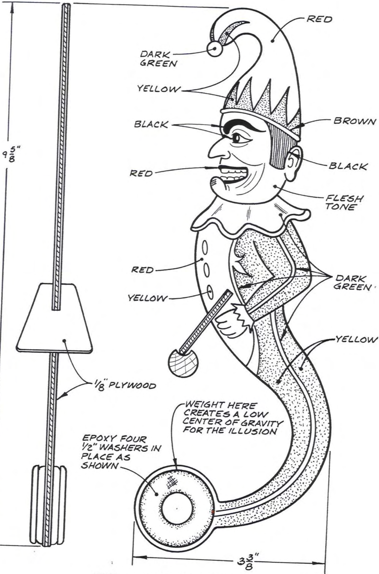
FULL-SIZE PATTERN
