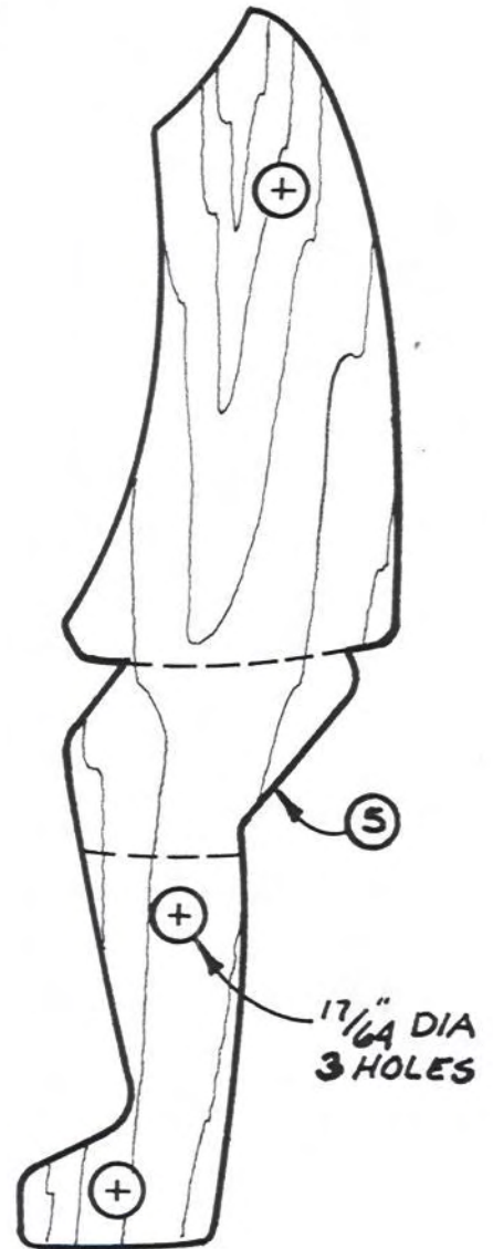
BODY SIDE 1/8" THICK (4 REQ'D)
