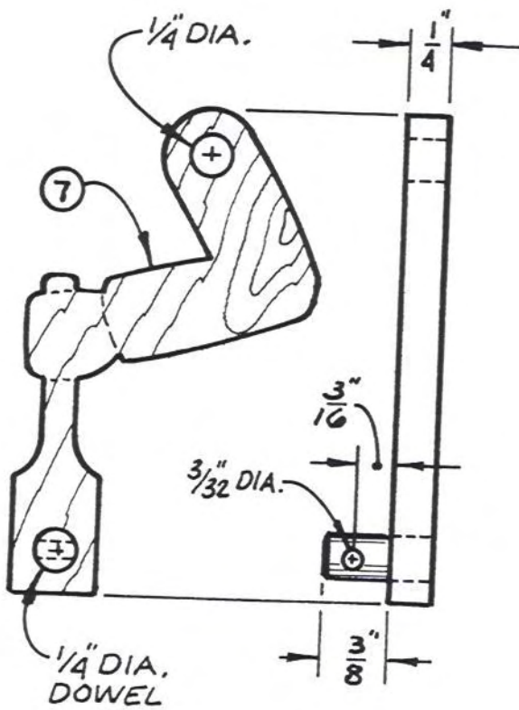
PIVOTING ARM (2 REQ'D)
