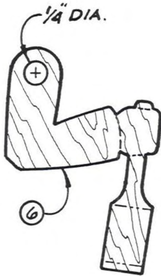
ARM 1/4" THICK (2 REQ'D)
